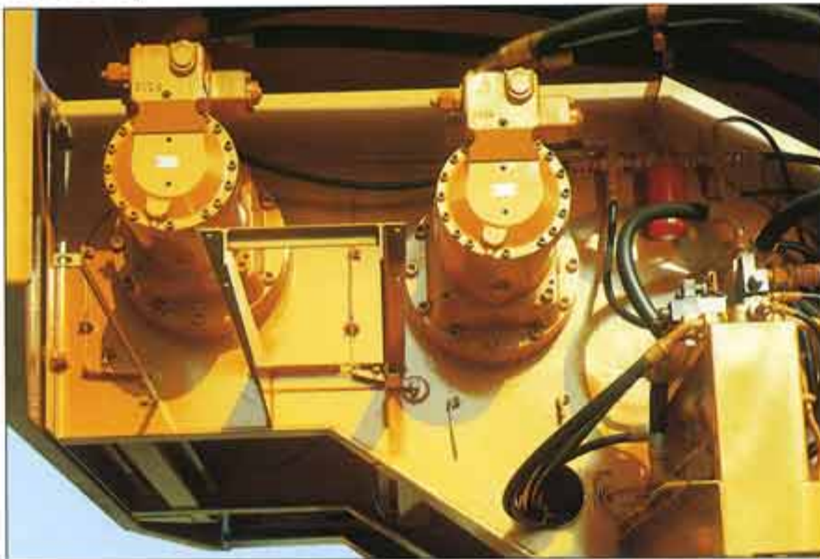
● Large main and auxiliary winches with separate motors for independent control of compound operations.
